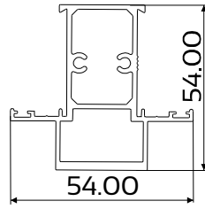
DIE No. W56796 Swift 38 54mm Mullion
