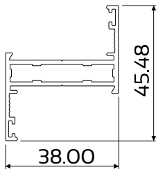
DIE No. W55717 Swift 38 Tubular Sash
