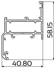
DIE No. W57508 Swift 38 Sash Euro
