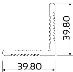
DIE No. W52538 Osborne Multi Corner Cleat
