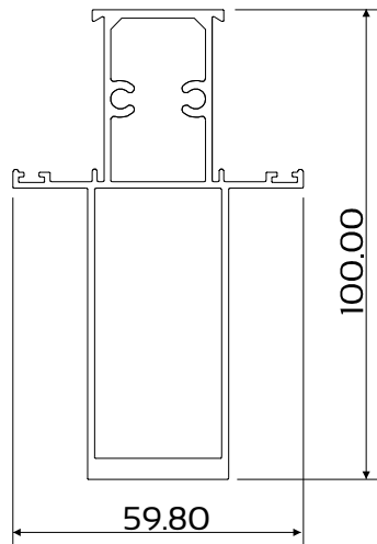
DIE No. W54454 Swift 38 100mm Mullion
