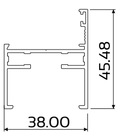
DIE No. W32070 Swift 38 Equal Leg Outer Frame
