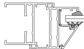
SECTION C-C Section not to scale
