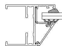
SECTION C-C Section not to scale
