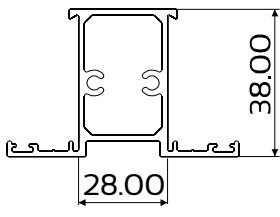
DIE No. W13268 Swift 38 Mullion / Transom
