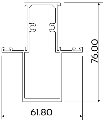
DIE No. W54455 Swift 38 76mm Mullion
