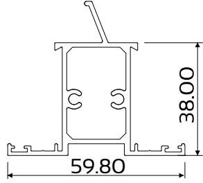
DIE No. W13408 Swift 38 Transom with Weather Bar
