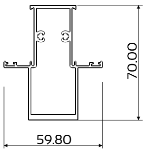
DIE No. W56797 Swift 38 70mm Mullion
