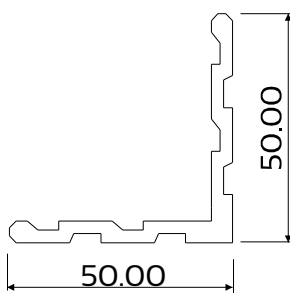
DIE No. W52695 50mm Corner Cleat
