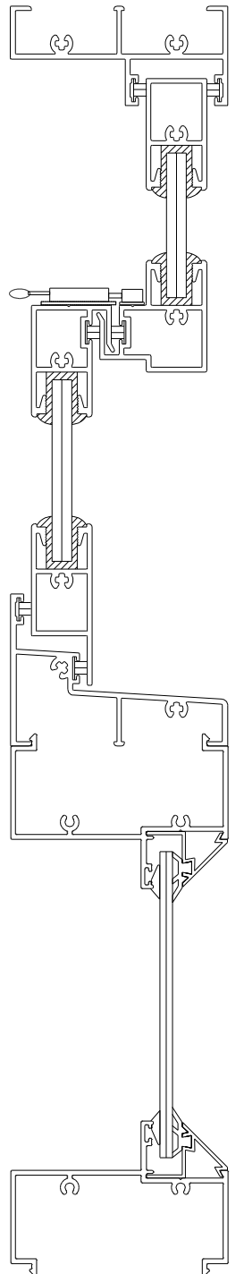
SECTION B-B Section not to scale
